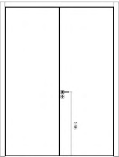
双开门正立面（推面） Front Elevation Of Double Doors (Push Panel)
