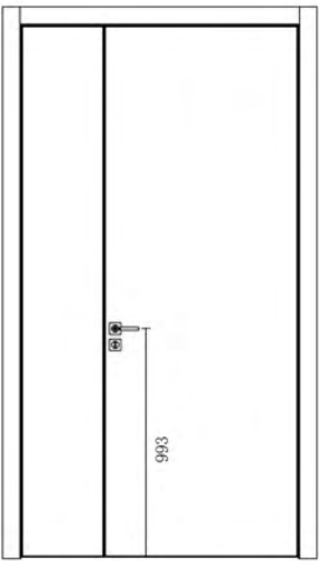
子母门正立面（推面） Front Elevation Of Parent And Child Door (Push Panel)
